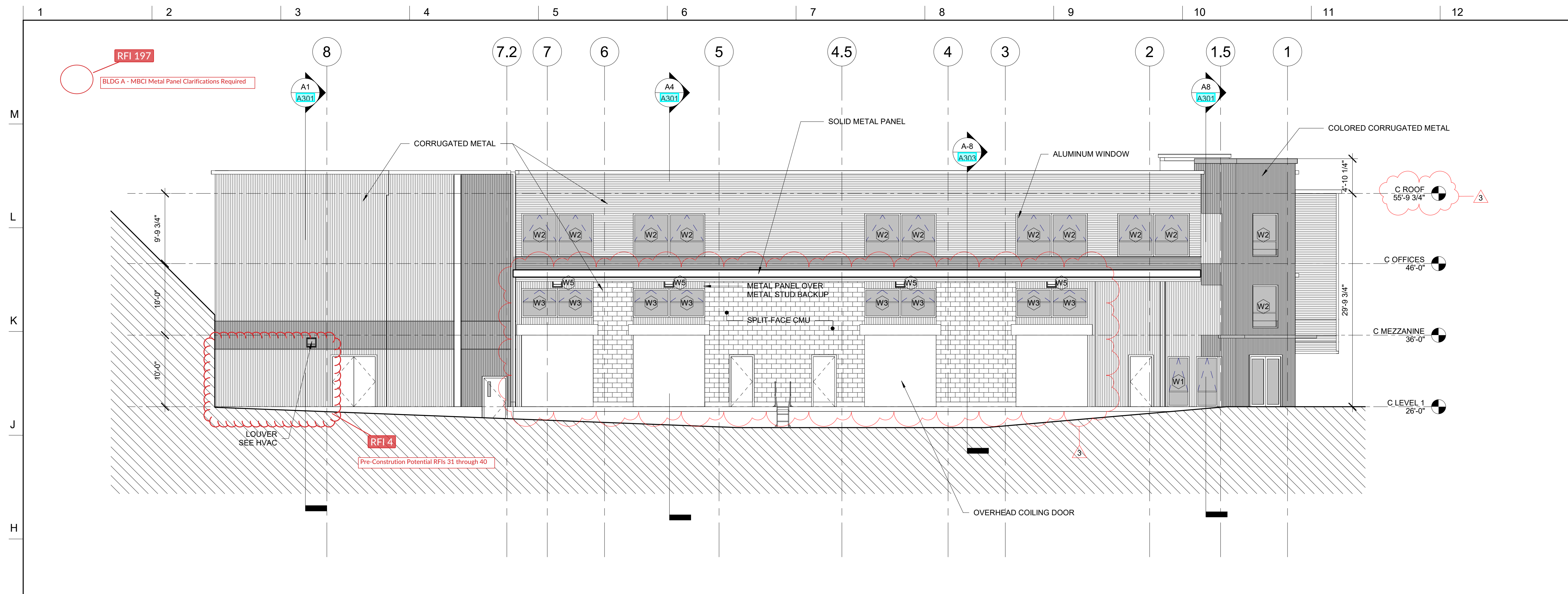
G1 PROPOSED SOUTH ELEVATION 1/8" = 1'-0"
